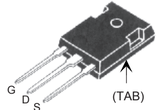
TO-247 (IXTH)
